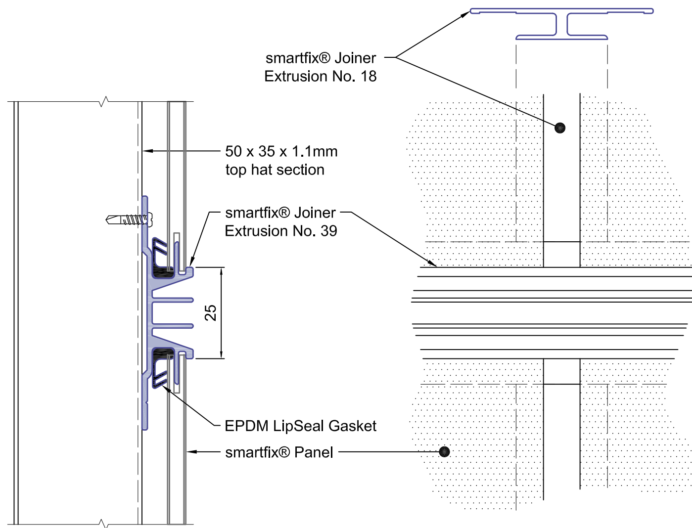
smartfix® Joiner Extrusion No. 39 Installed Horizontally
