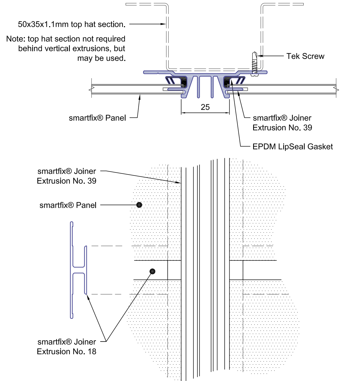
smartfix® Joiner Extrusion No. 39 Installed Vertically
