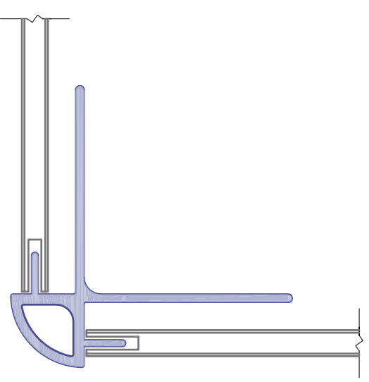
EXTRUSION No. 6
