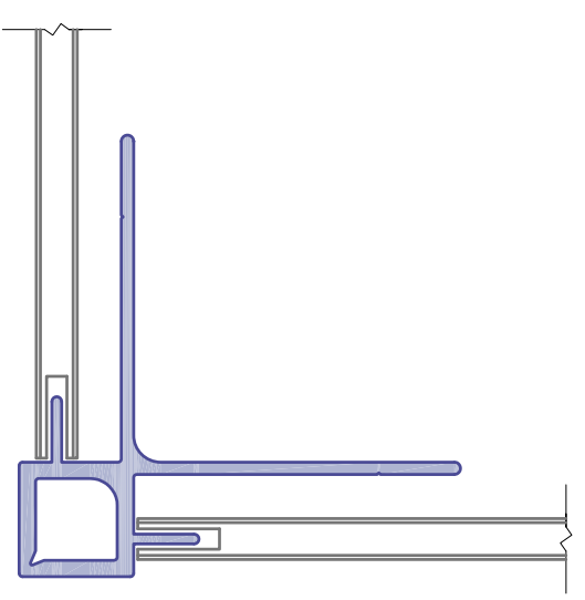
EXTRUSION No. 7
