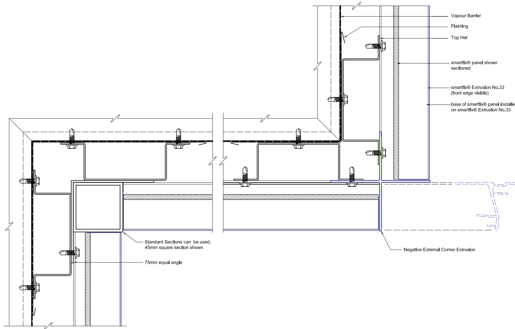
A-A - SECTION PLAN DETAIL
